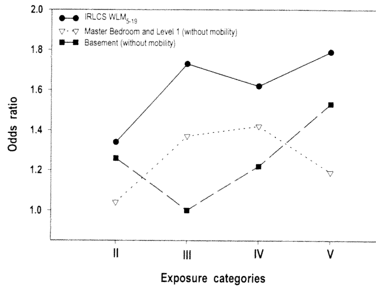
FIGURE 2. Plots of risk estimates for the all cases and controls calculated by using alternative radon exposure estimate scenarios, IRLCS, Iowa, 1993–1997. IRLCS odds ratios, as reported in table 4, are presented for comparison. The odds ratios plotted as the master bedroom and living area are based on a simple arithmetic average of the radon measurements from the two rooms. The odds ratios plotted for the basement are based on the average yearlong radon concentration in the basement without consideration of retrospective subject mobility. An average home occupancy of 70 percent time was assumed for the master bedroom and level 1 (living area) plot and the basement plot.
